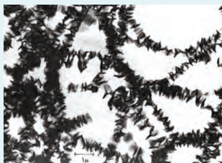
Figure 1. Transmission electron micrograph of 'shish-kebab' crystal structure of polyethylene, produced by an elongational flow-field (Mackley and Keller, Pure Appl. Chem. , 39, 193, 1974)
